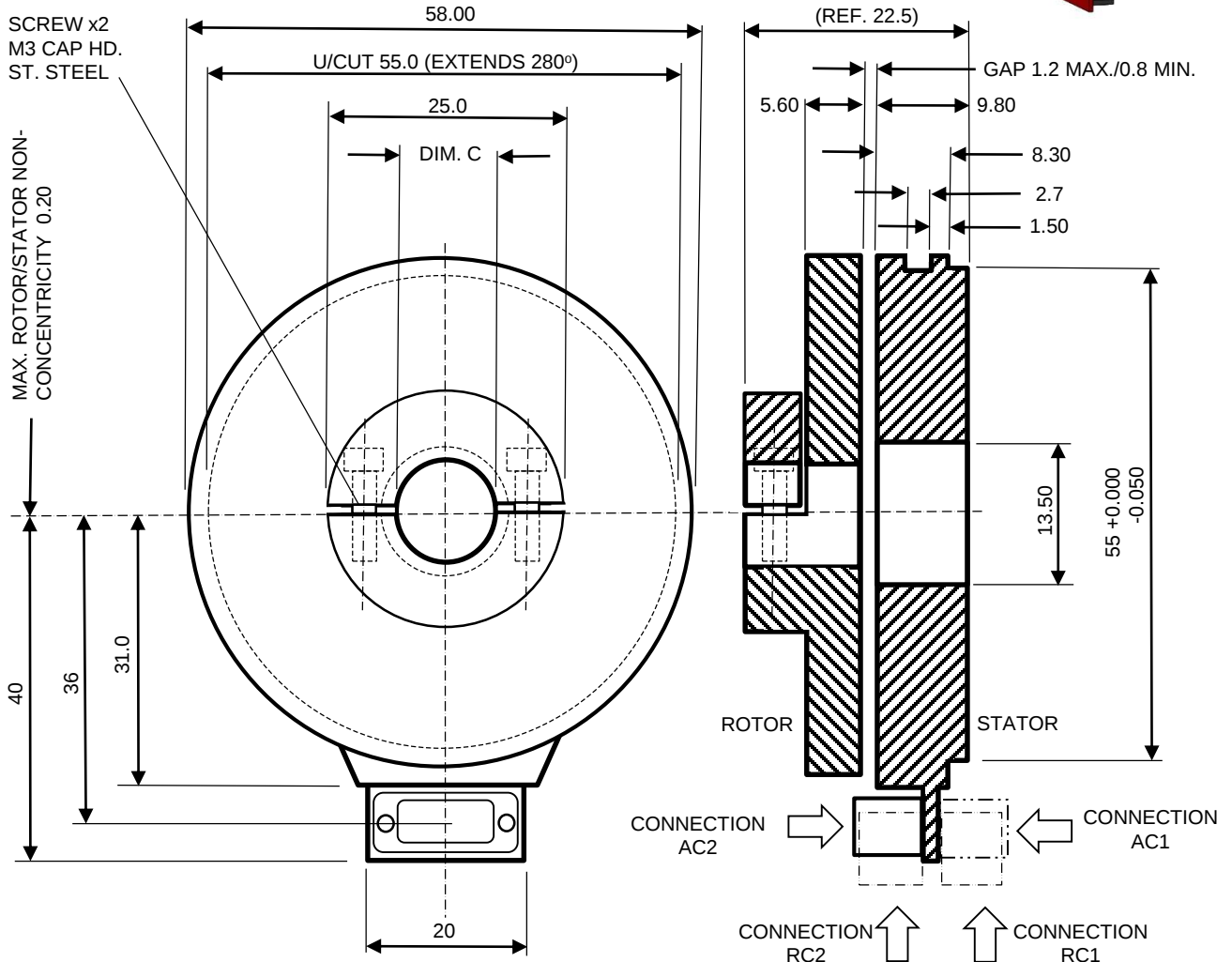
SCRAP VIEW SHOWING VFLx CONNECTION
